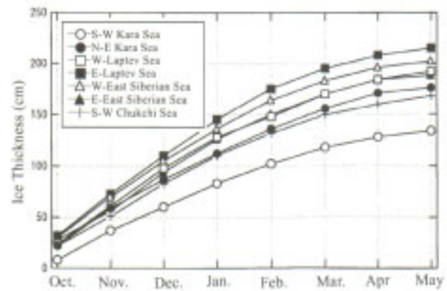
Figure 4.2-4 Growth of sea ice in winter
