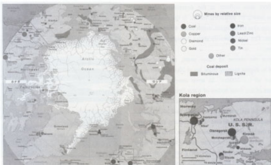
Distribution of mineral resources in the Arctic (revision to the Atlas of the Polar Regions)
