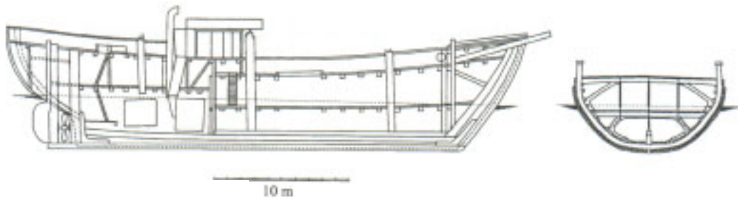
Figure 4.1-1 The Fram
