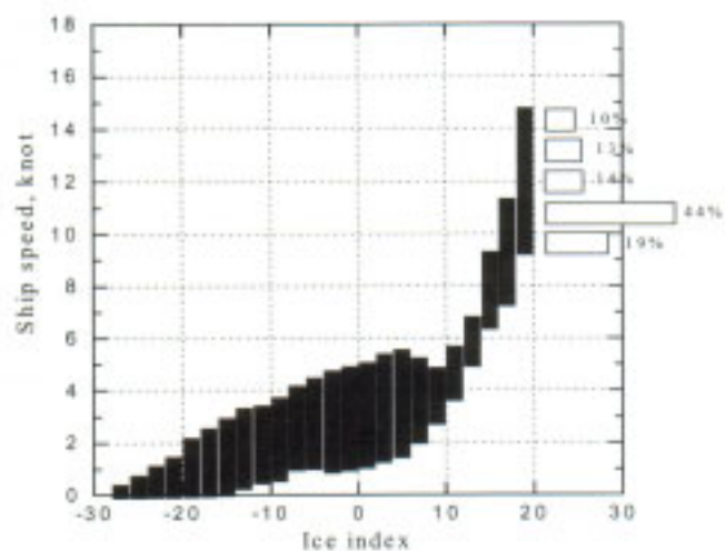
Figure 4.4-4 Ship speed distribution and ice index for 50BC
