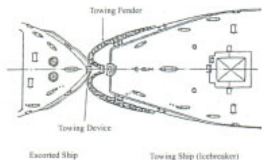
Figure 4.1-10 Stern notch
