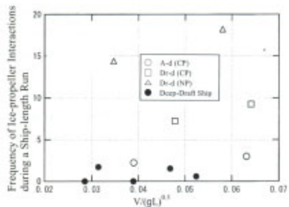
Figure B-19 Frequency of interactions between ice and propeller
