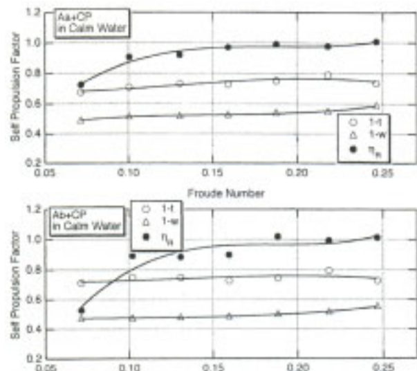
Figure B-9 Self-propulsion factors in calm water
