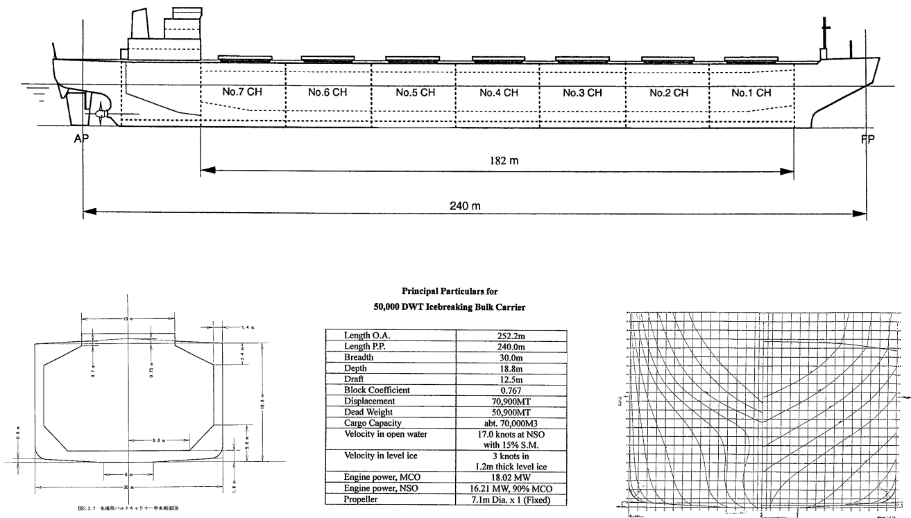
Figure C-14 General arrangement of the 50,000DWT icebreaking bulk carrier (50BC)
