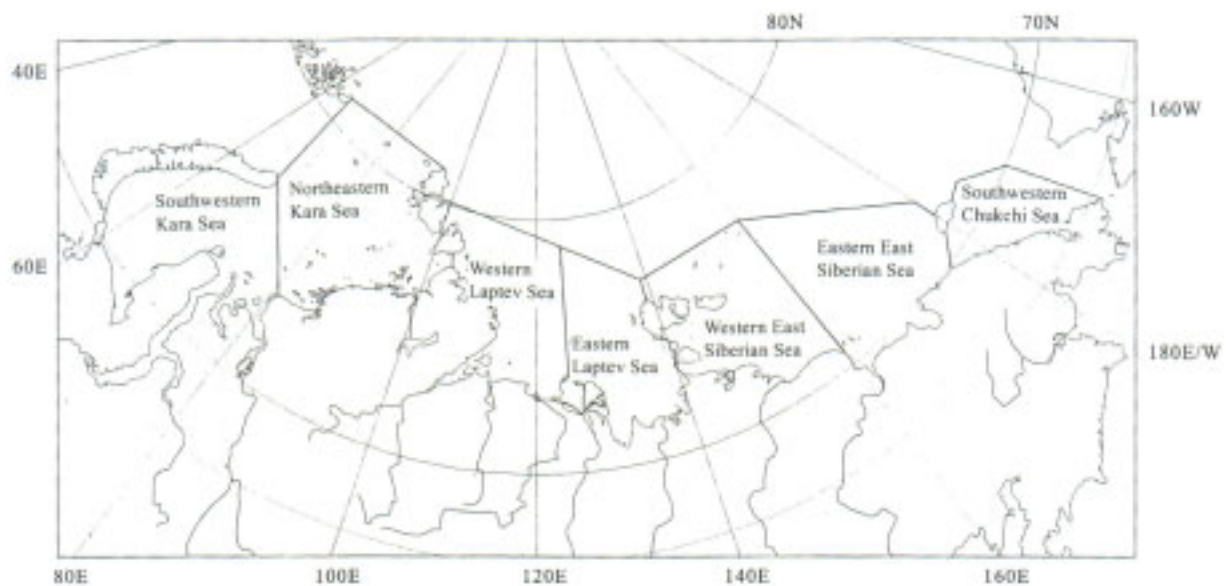
Figure 4.2-2 Ice-region boundaries for the Russian maritime Arctic
