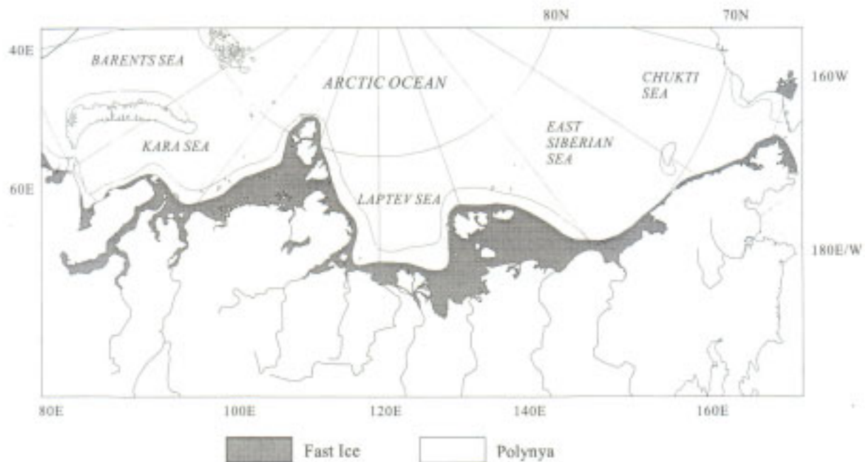
Figure 4.2-3 Fast ice
