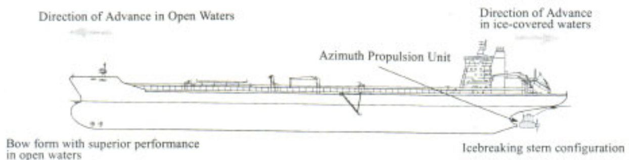
Figure 4.1-15 DAS concept
