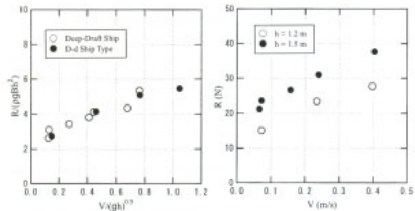
Figure B-18 Results of resistance tests in level ice
