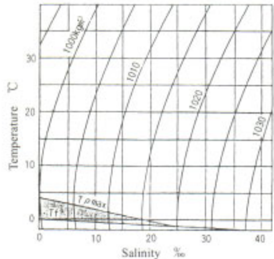
Temperature-density-salinity diagram of sea water
