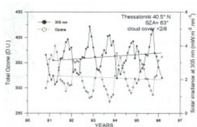
Yearly changes of total ozone and solar irradiance at 305nm(UVB) (Zerefos,1997)
