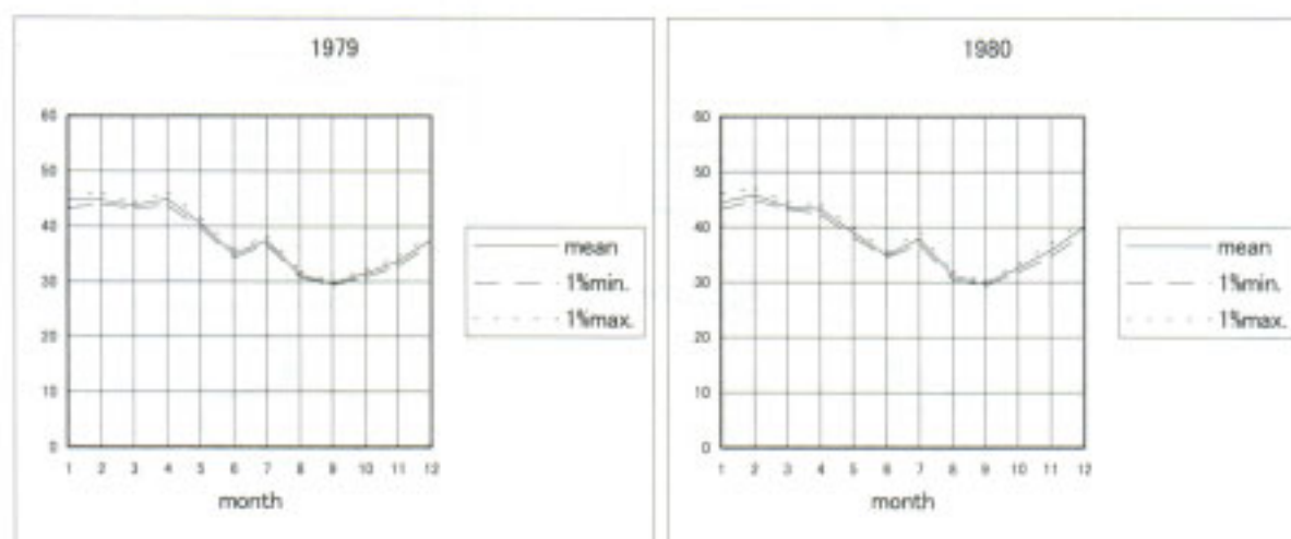
Figure 4.4-8 Example of voyage-days for 40BC (1979, 1980)
