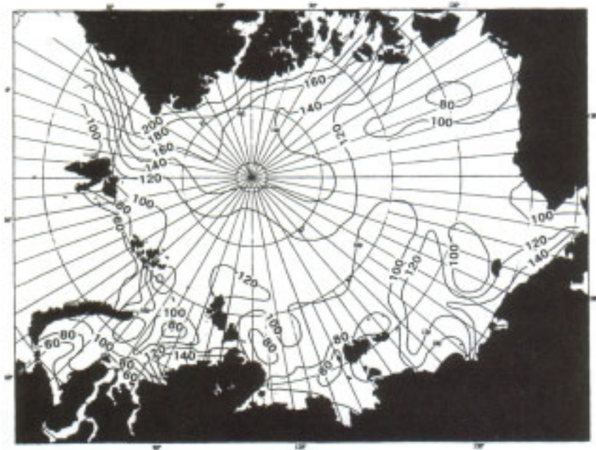
Maximum snow cover in the vicinity of pressure ridges in April (cm)
