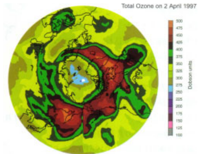
Ozone distribution in the northern hemisphere (NASDA/NASA,1998)
