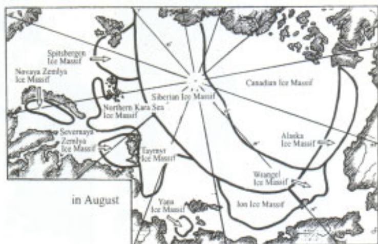
Ice massifs in the Arctic Ocean (Romanov,1994)
