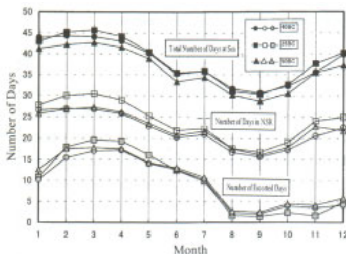
Figure 4.4-9 Average number of voyage-days for each of the three ships; full voyage, voyage in NSR and escorted voyage (average values from 1957 to 1990)
