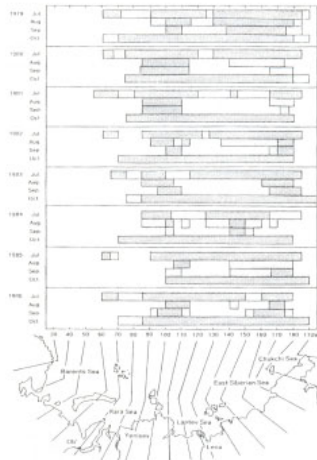
Sea ice concentrations in summer in the NSR regions (Ono,1996)
